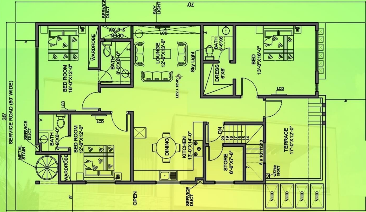
A-02 FIRST FLOOR PLAN
