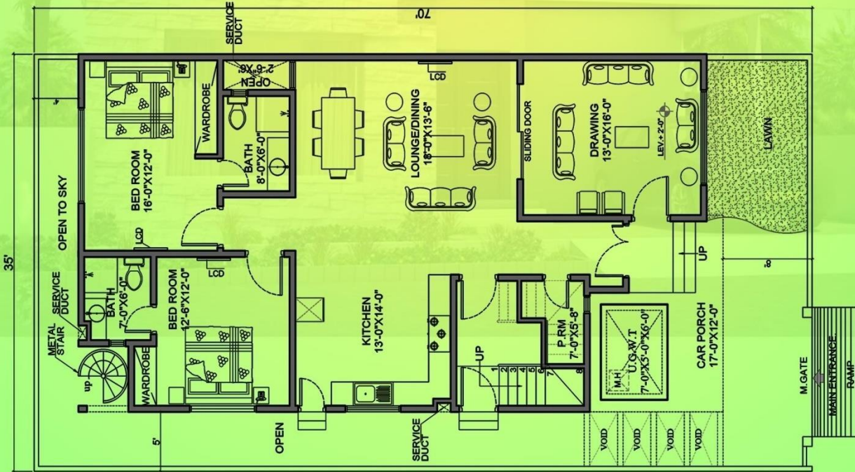
A-01 GROUND FLOOR PLAN
